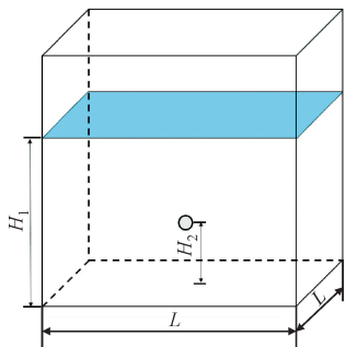
图 2 静水中单气泡上升算例初始状态示意图 Fig.2 Schematic diagram of the initial state for the single bubble rising in still water
