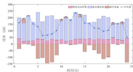
(c) IES冷平衡
