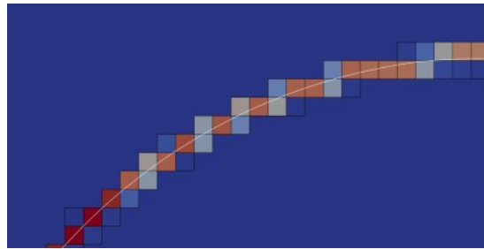
(e) A_{PLIC}/V_{cell}
