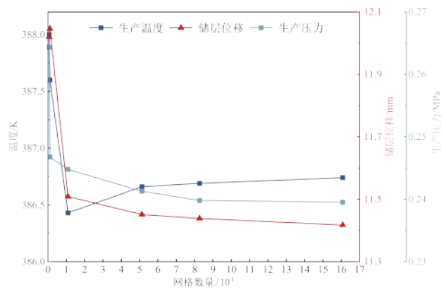
图2 网格独立性验证 Fig. 2 Grid independence verification
