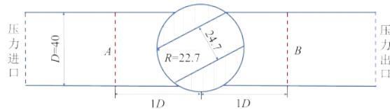
图7 球阀的几何结构 Fig. 7 The geometry of the ball valve
